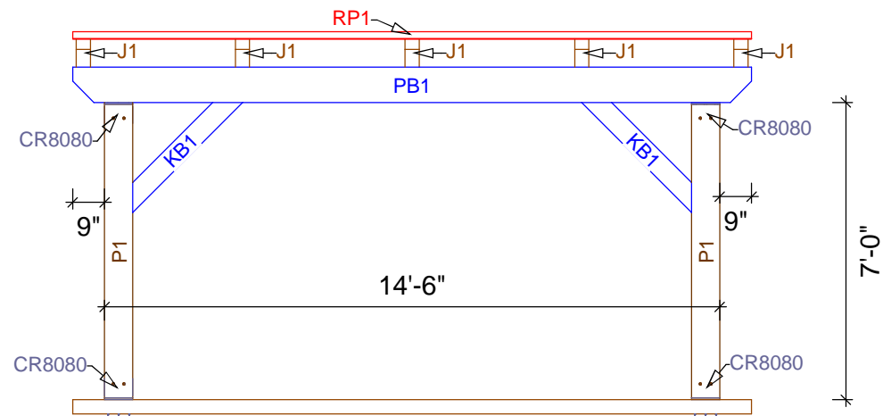
Front
