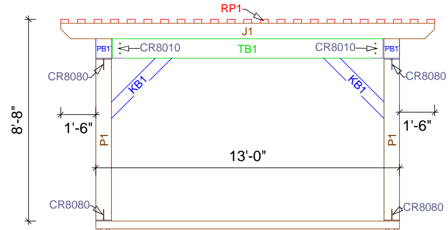
Side
