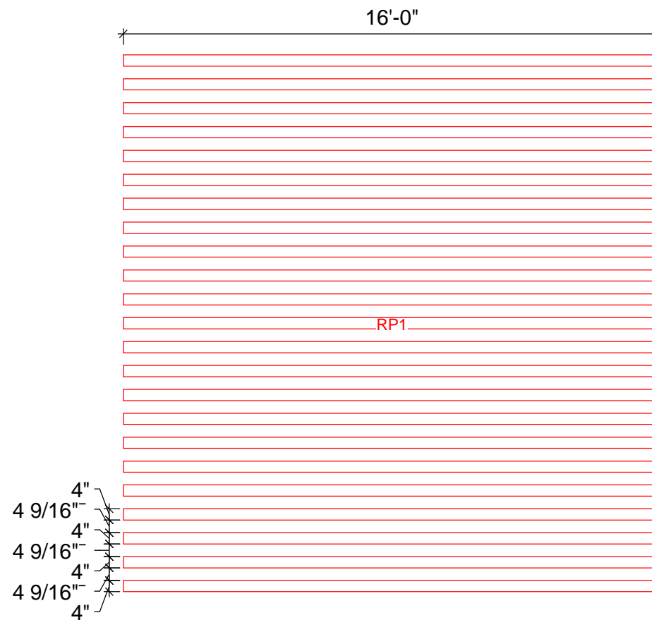
Purlin Layout
